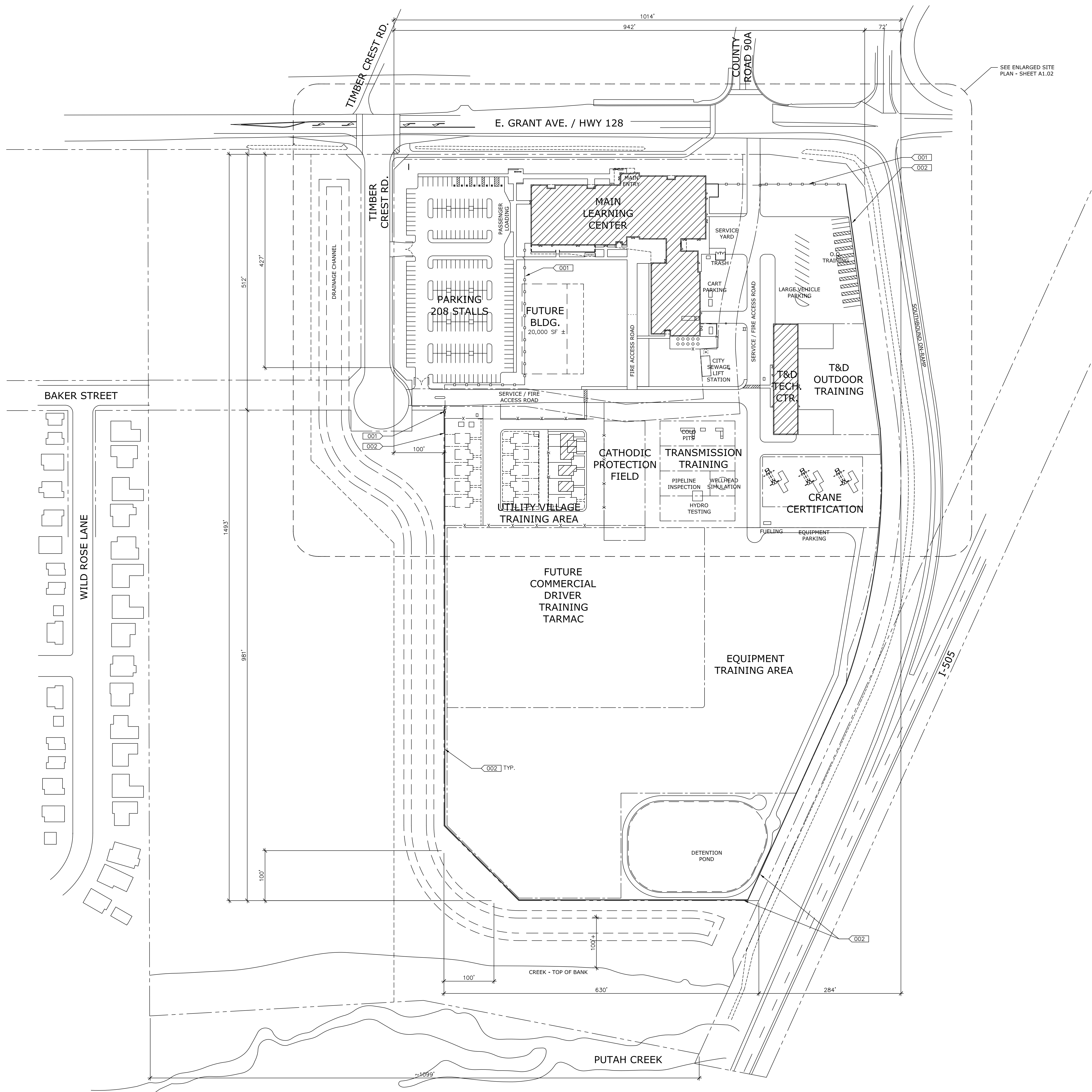
1 OVERALL SITE PLAN
